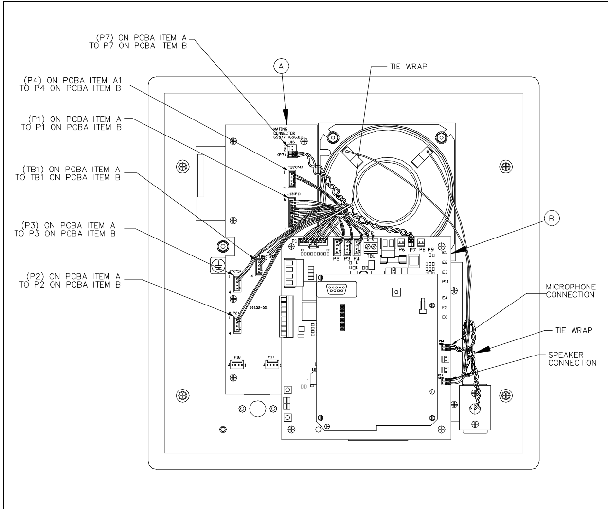
Figure 4. No. 295-702F/W Wiring Detail
