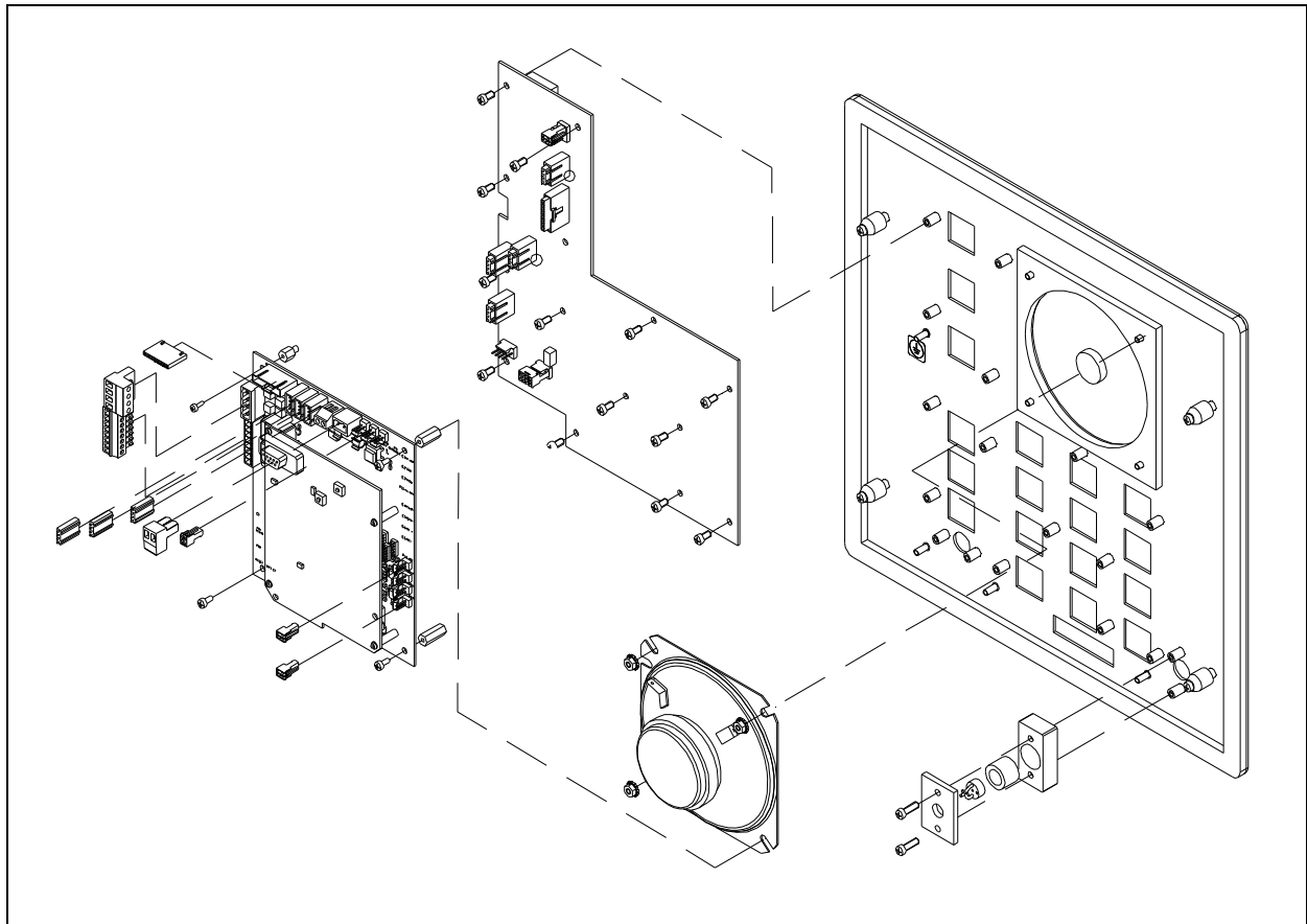
Figure 3. No. 295-702F/W Assembly Detail
