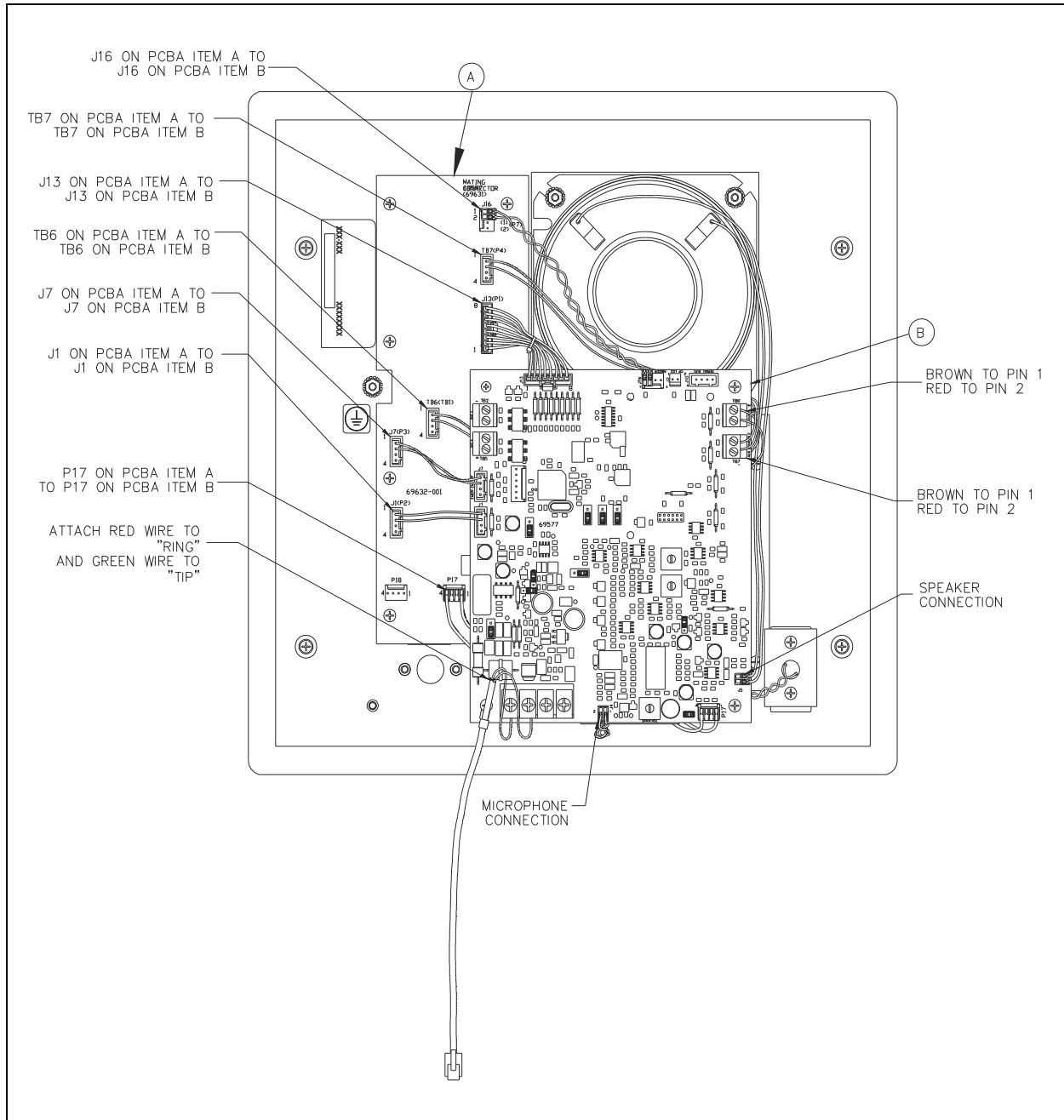
Figure 2. No. 295-001F/W Wiring Detail
