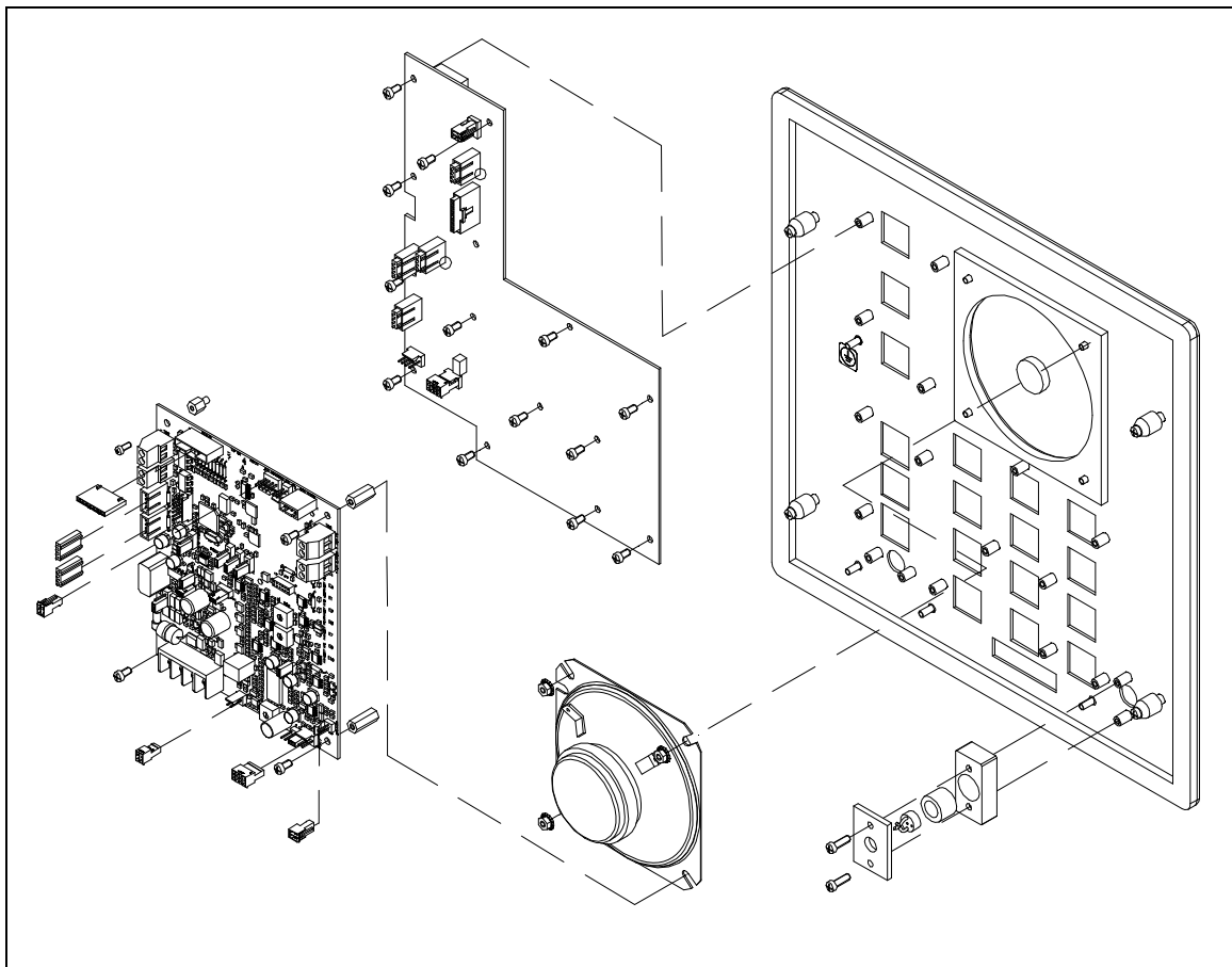
Figure 1. No. 295-001F/W Assembly Detail
